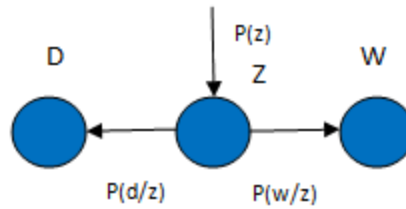
Figure 3. Graphical representation of the aspect model in a symmetric form. D represents samples, W tokens and Z components.
