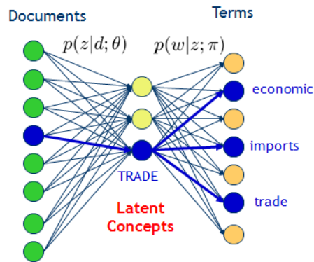
Figure 1. Schematic representation of PLSA general structure. It shows the latent topics that links documents and words into common topics with the associated probabilities. Source: [13].
